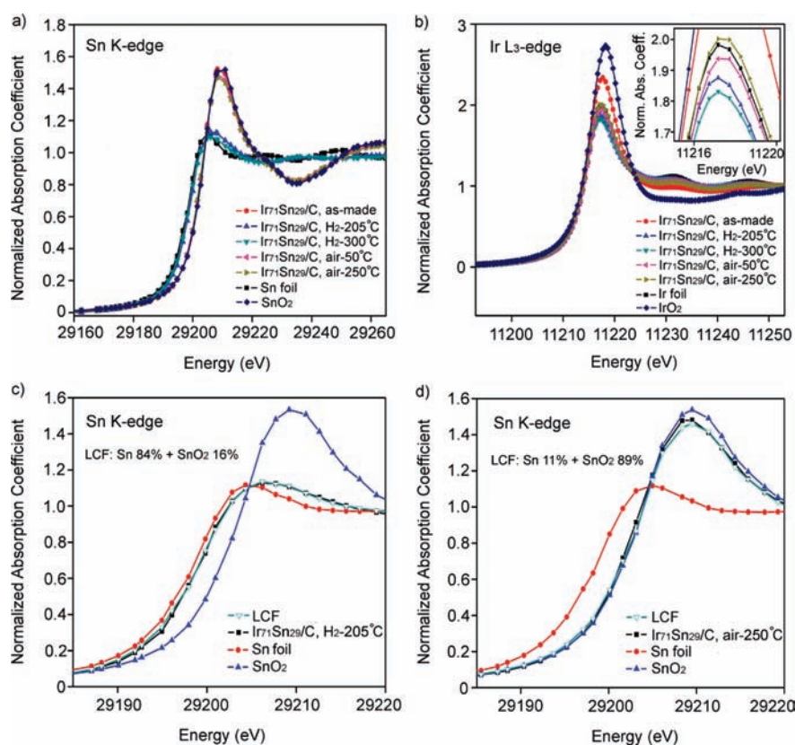
Figure 3. Selected XANES spectra of (a) Sn K-edge and (b) Ir L_3 -edge of \text{Ir}_{71}\text{Sn}_{29}/\text{C} during the reduction in \text{H}_2/\text{He} flow and oxidation in air flow at different temperatures; (c) LCF of \text{Ir}_{71}\text{Sn}_{29}/\text{C} after reduction at 205 °C under \text{H}_2/\text{He} flow and (d) LCF fit of \text{Ir}_{71}\text{Sn}_{29}/\text{C} after oxidation at 250 °C under air flow.
