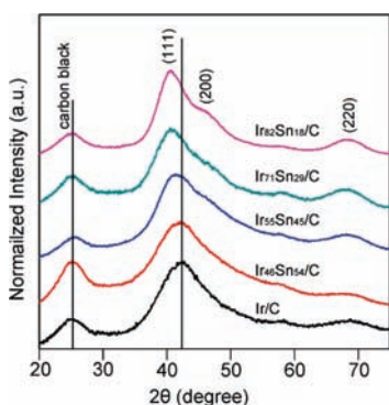
Figure 2. XRD patterns of carbon-supported Ir, \text{Ir}_{46}\text{Sn}_{54} , \text{Ir}_{55}\text{Sn}_{45} , \text{Ir}_{71}\text{Sn}_{29} , and \text{Ir}_{82}\text{Sn}_{18} nanoparticles after reduction at 205\text{ }^\circ\text{C} under \text{H}_2/\text{Ar} flow.
