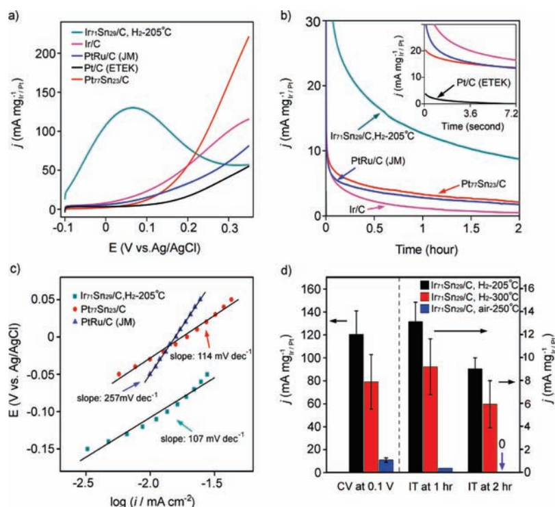
Figure 5. Electrochemical measurements of carbon-supported Ir 71 Sn 29 , Ir, and Pt 77 Sn 23 and Pt (EETEK), PtRu (JM) catalysts: (a) CVs from -0.1 \sim 0.35 V and (b) current density vs time measurements at 0.1 V in 0.5 M of H 2 SO 4 /0.5 M of ethanol electrolyte, (c) Tafel plot for ethanol electrooxidation on Ir 71 Sn 29 /C, Pt 77 Sn 23 /C, and PtRu (JM) catalysts in 0.5 M of H 2 SO 4 /0.5 M of ethanol electrolyte at scan rate of 1 mV s -1 (data extracted from LSV measurements), and (d) comparisons of CV and current density vs time measurements between Ir 71 Sn 29 /C reduced in H 2 /Ar at 205 °C, Ir 71 Sn 29 /C reduced in H 2 /Ar at 300 °C, and Ir 71 Sn 29 /C oxidized in air at 250 °C conducted at the same conditions as in (a) and (b).
